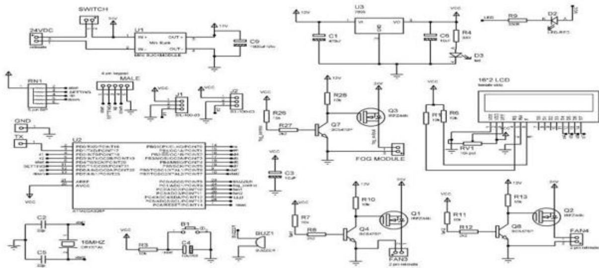
Figure 2: Circuit Diagram
