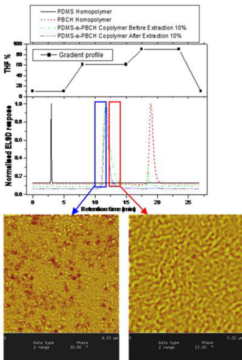
Figure 1: GEC result for PDMS, PBCH homopolymers and PDMS-PBCH random multiblock copolymer with 10% PDMS content, when the above gradient profile was used and AFM images taken for each a signed fraction of the copolymer
